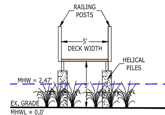
SECTION VIEWS SCALE: 1"=10'
